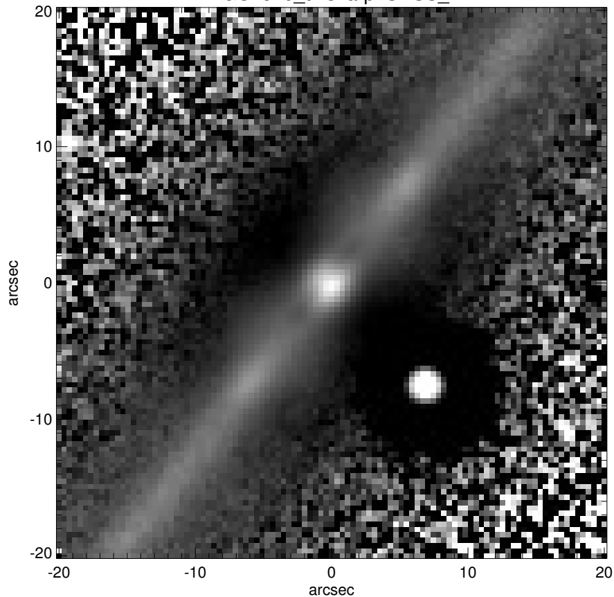
NGC2826_unsharp SDSS_r
