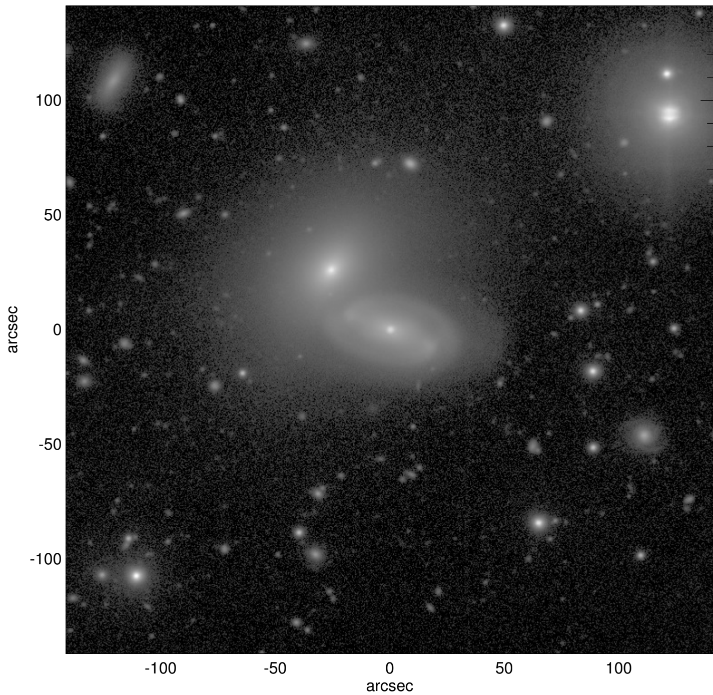
NGC0078A
