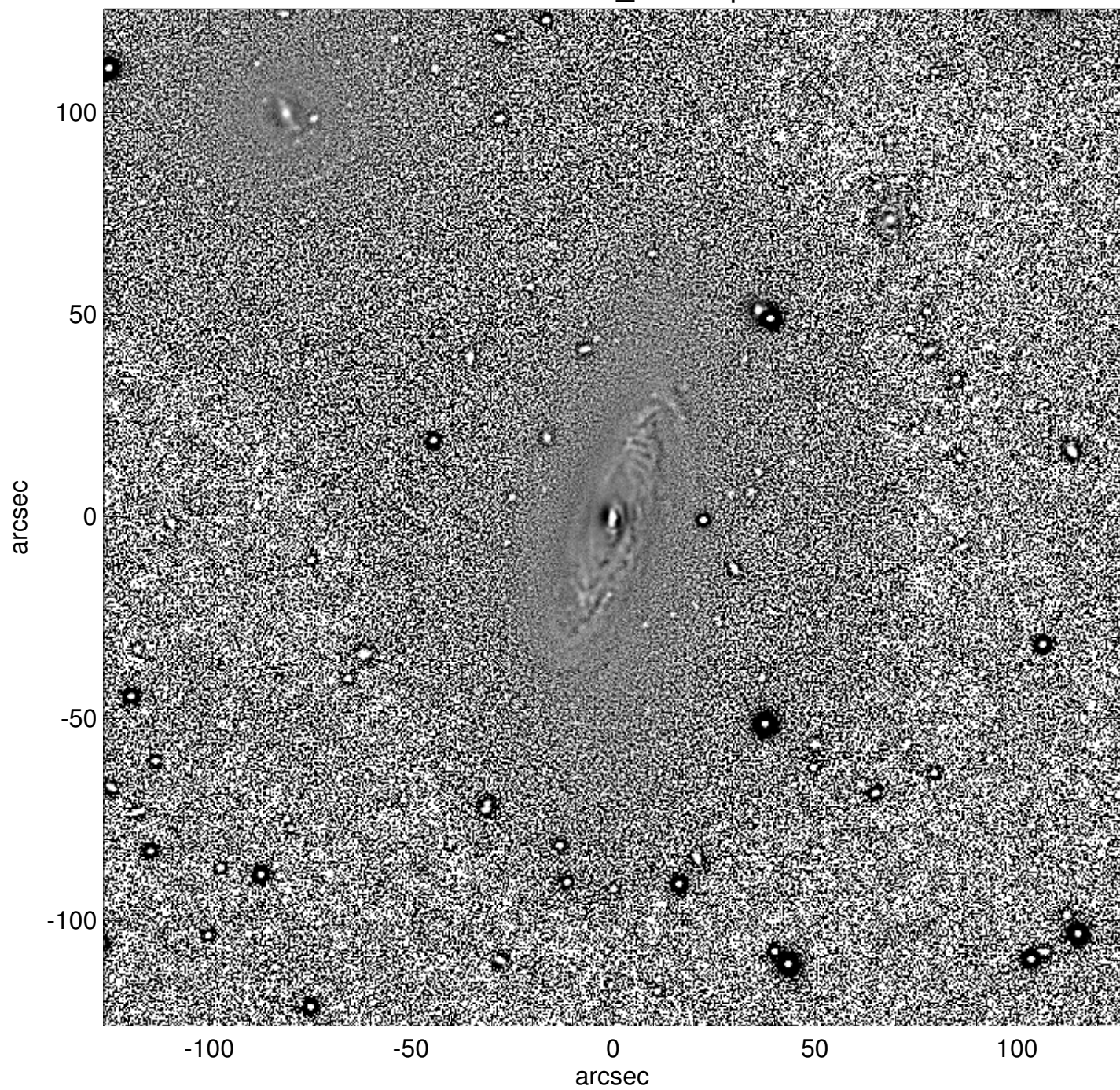
NGC0192_unsharp
