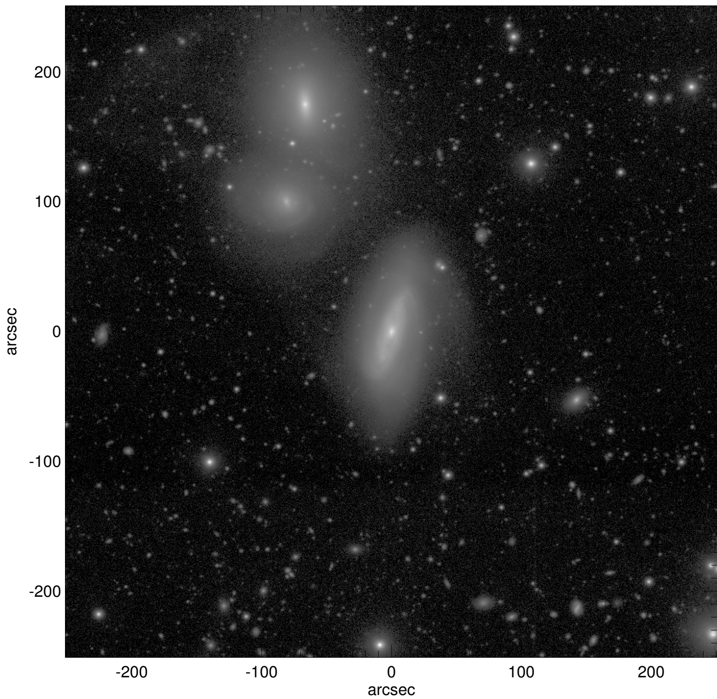
NGC0192
