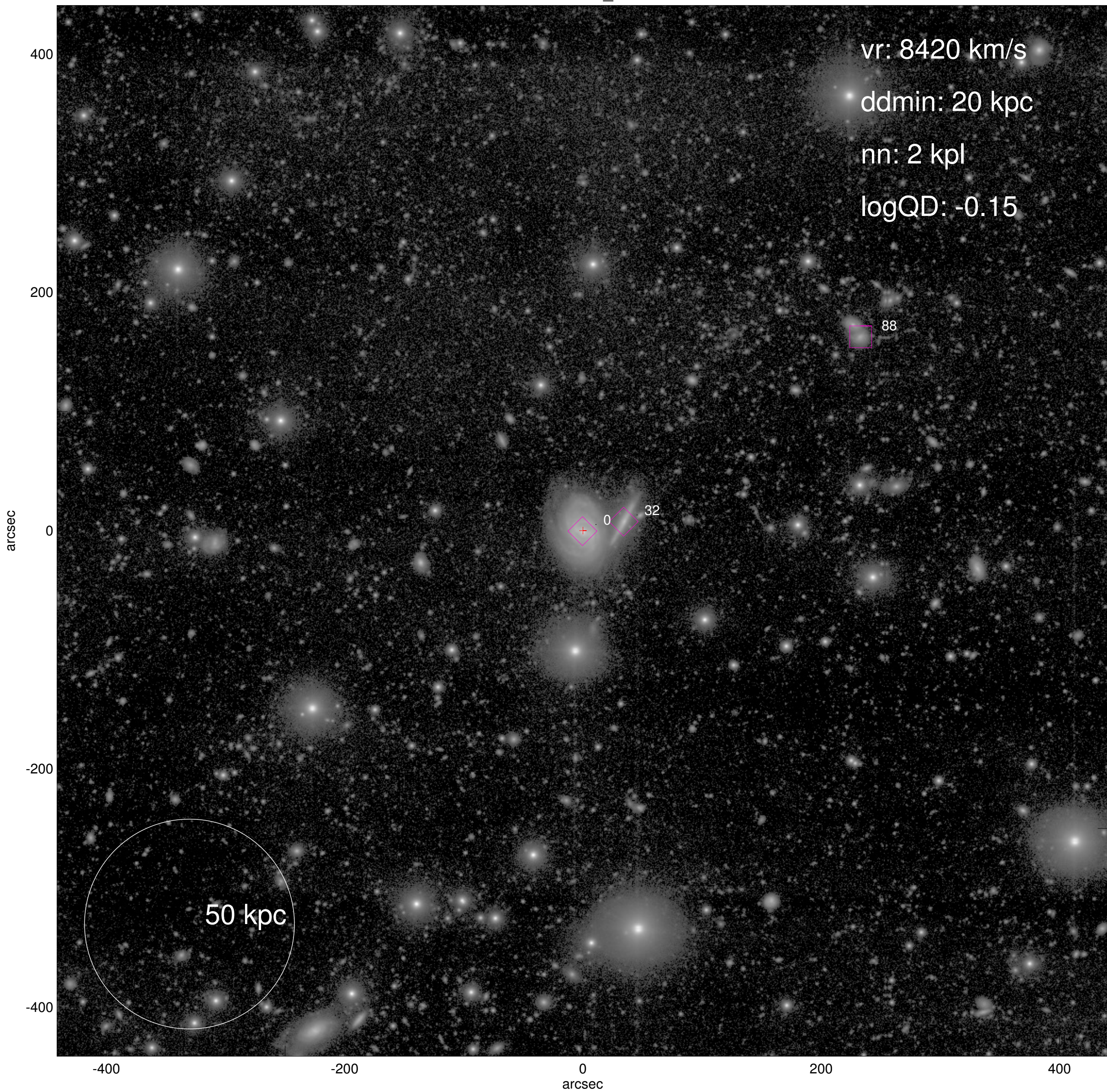
UGC02324_wide
