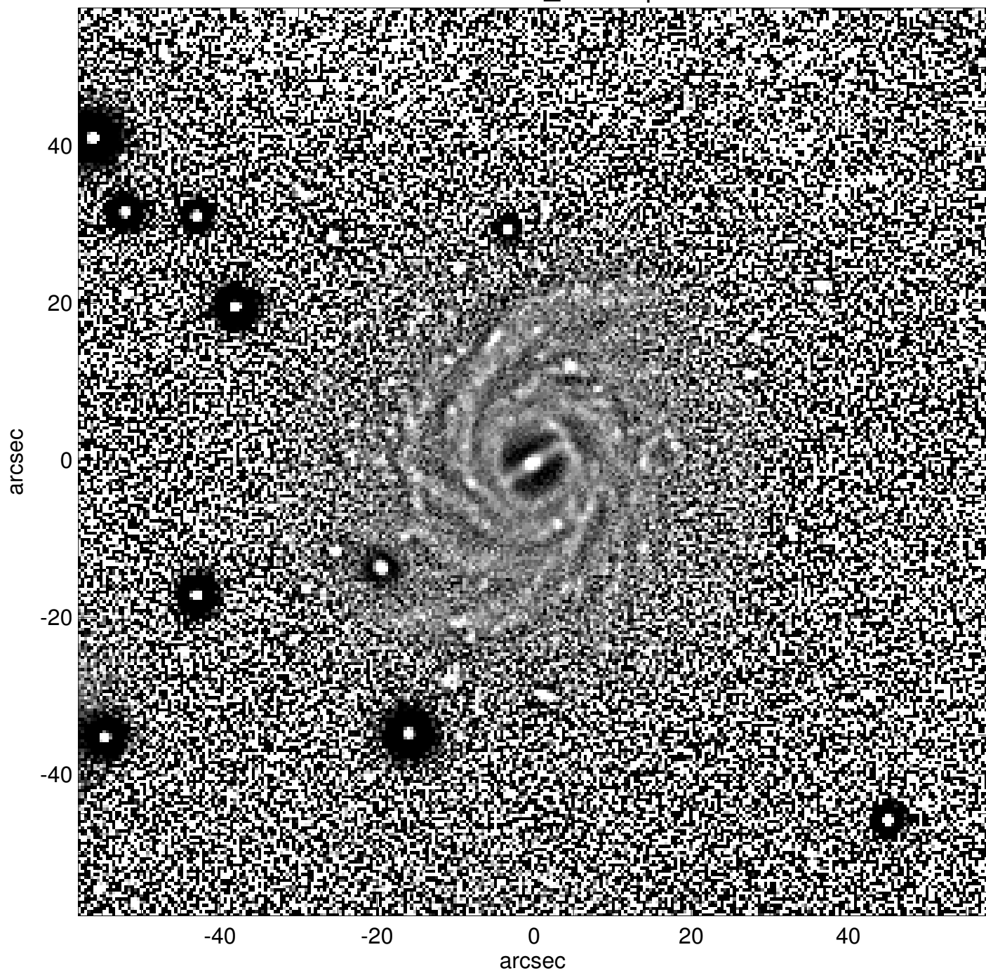
UGC02705_unsharp
