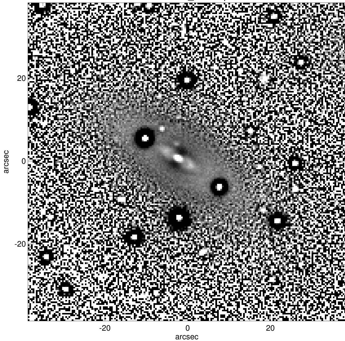
NGC6959_unsharp
