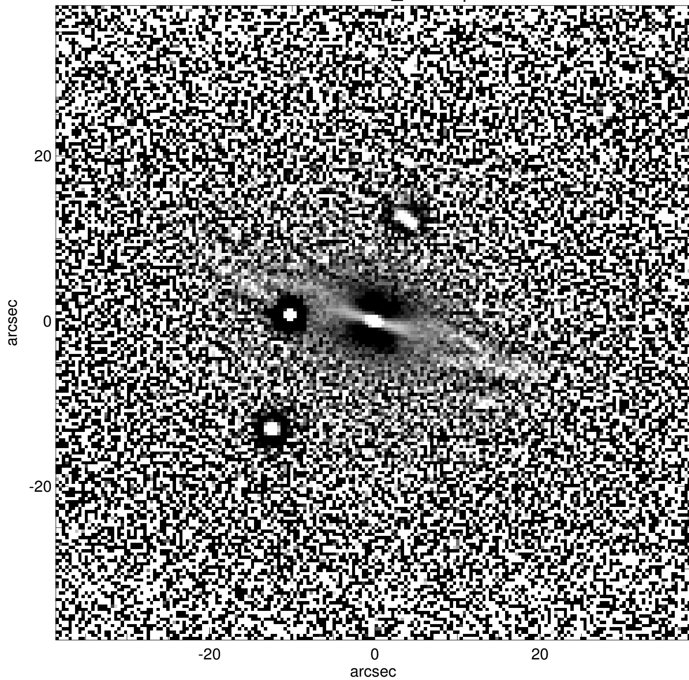
PGC1128060_unsharp
