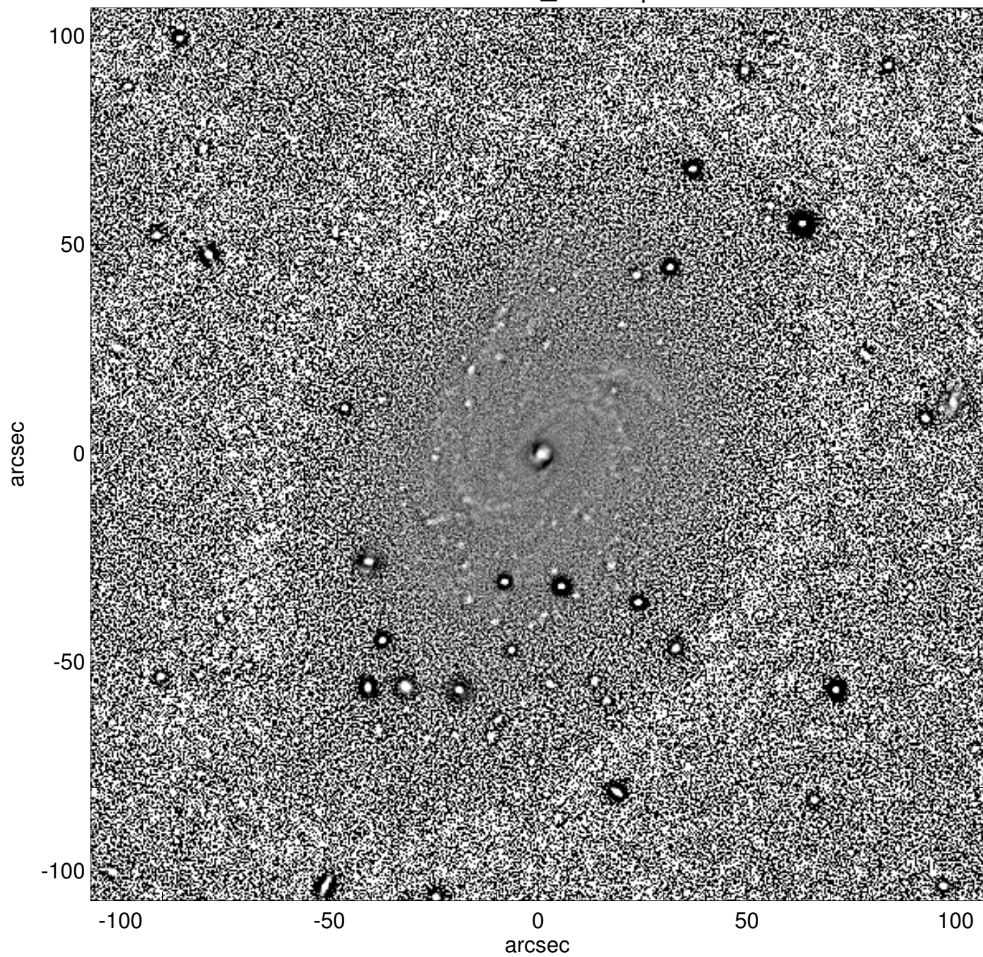
NGC0201_unsharp
