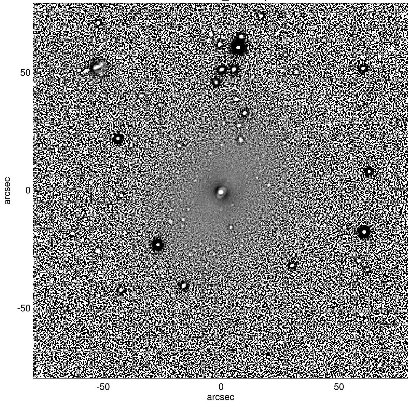
NGC0426_unsharp
