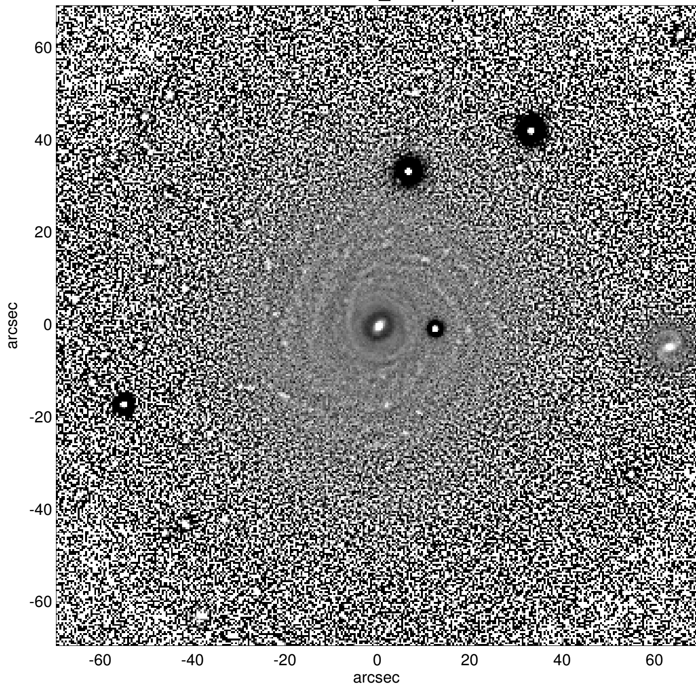
NGC0863_unsharp
