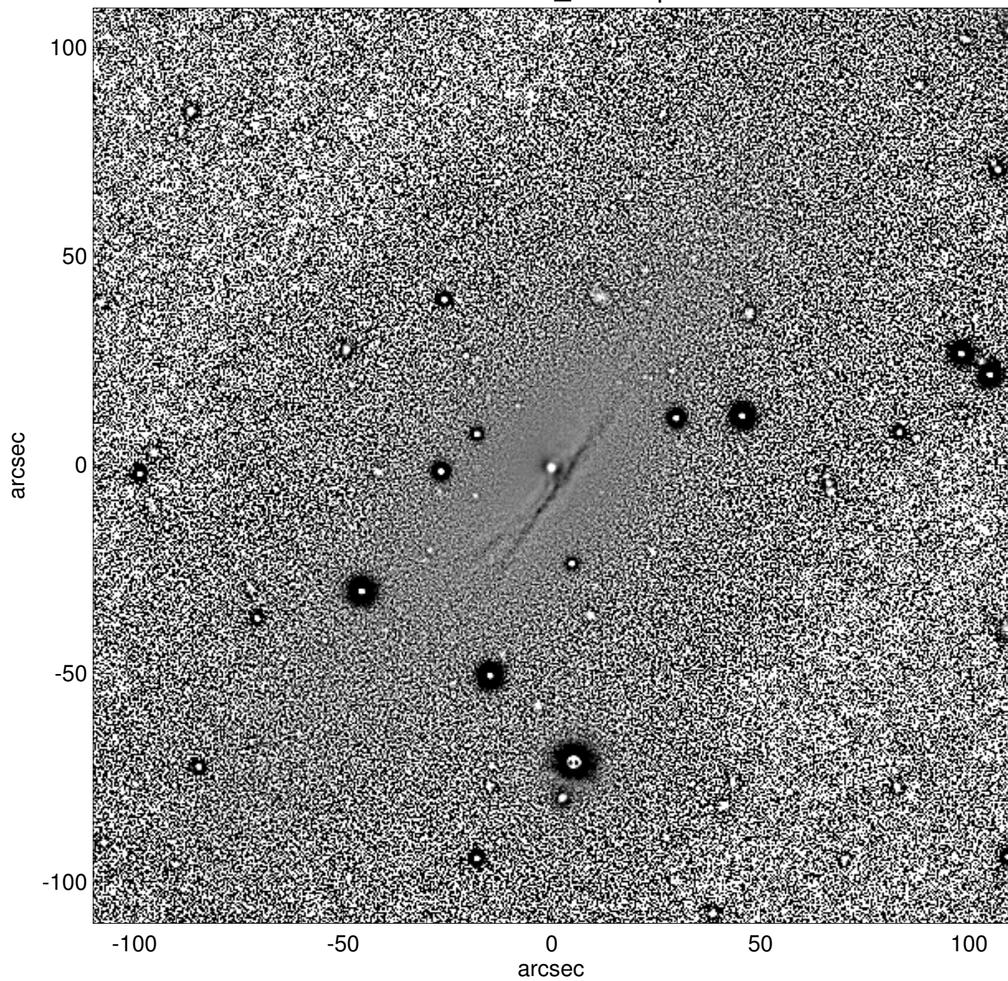
NGC1194_unsharp
