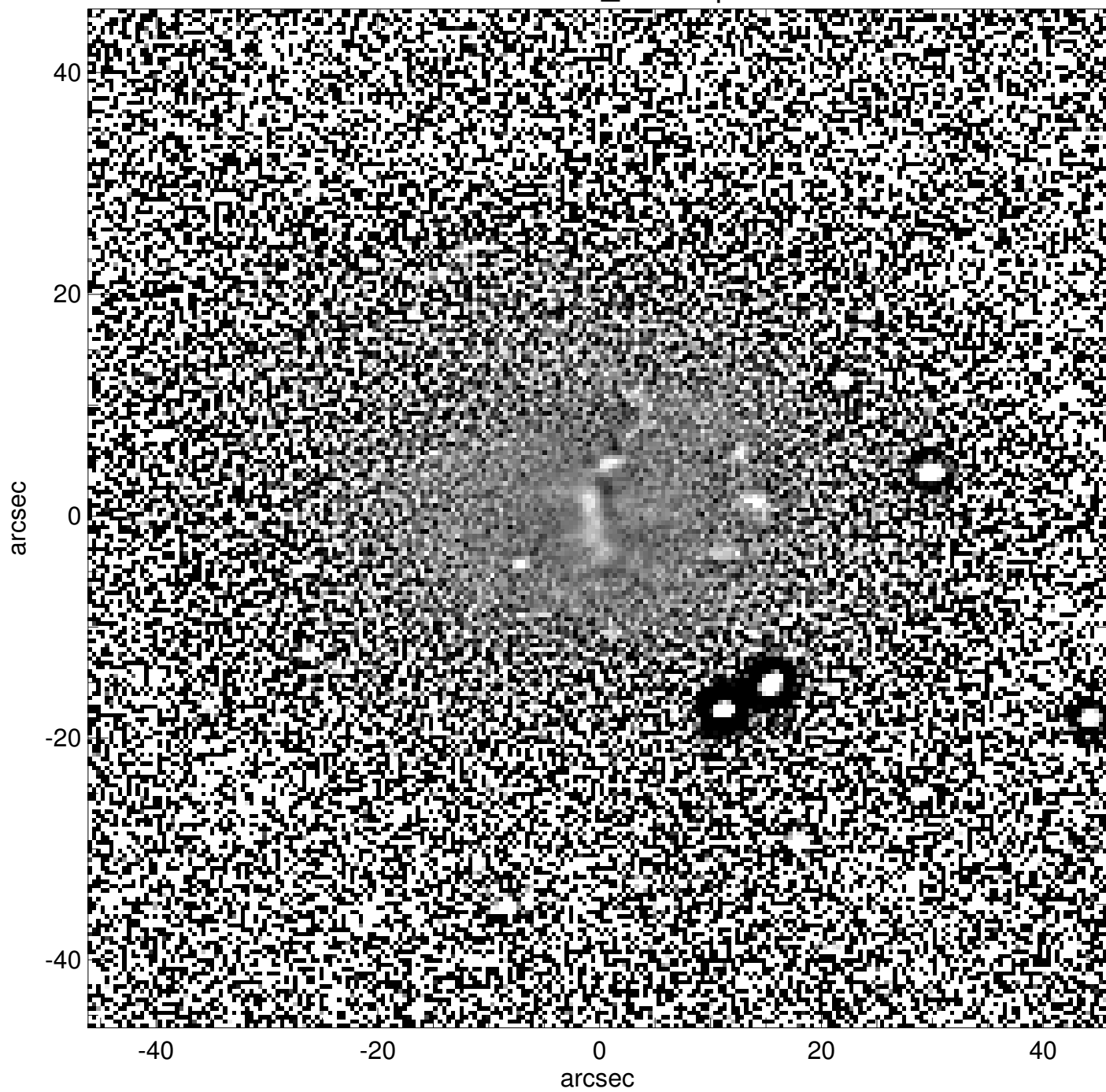
NGC7401_unsharp
