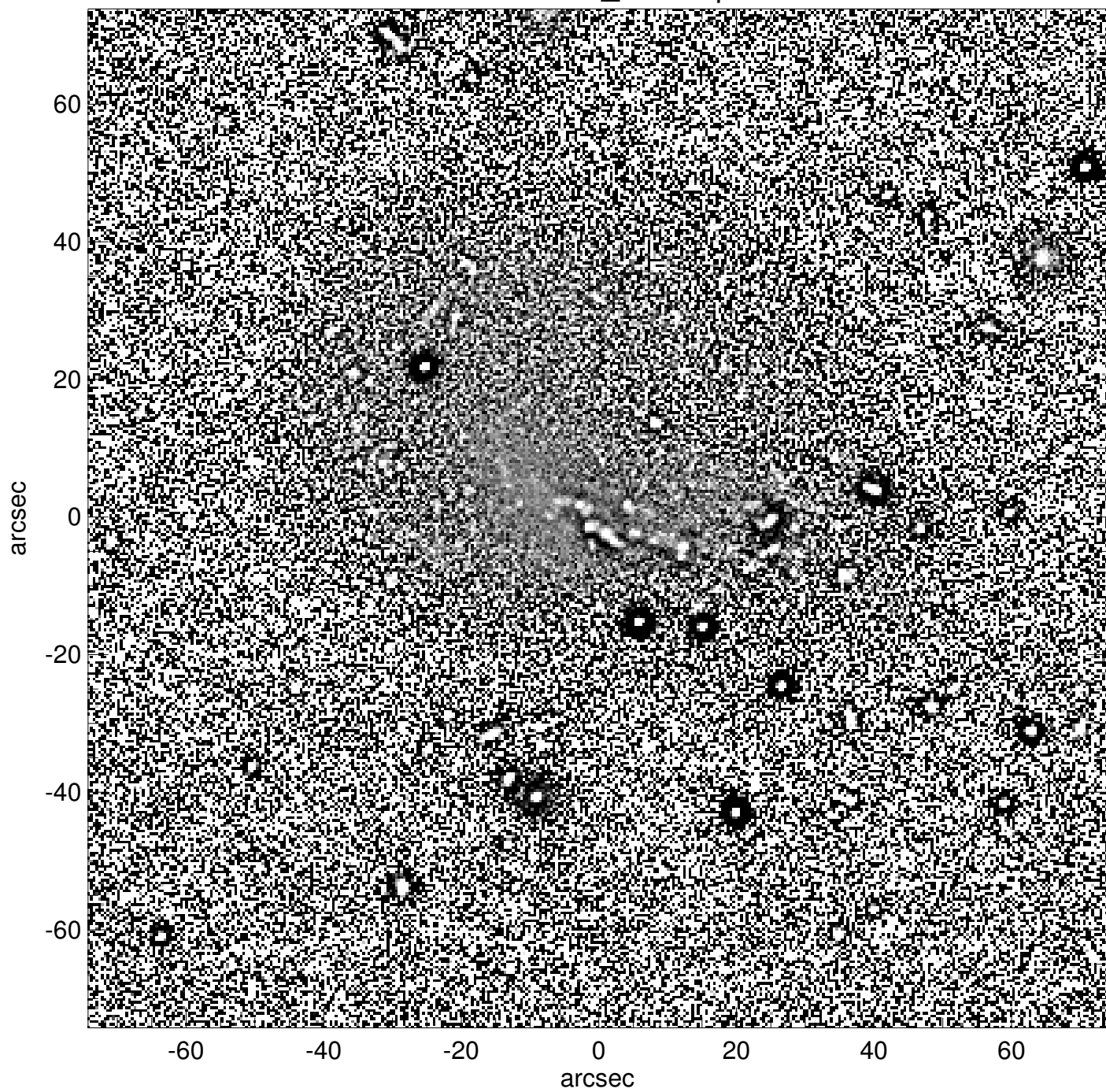
NGC7667_unsharp
