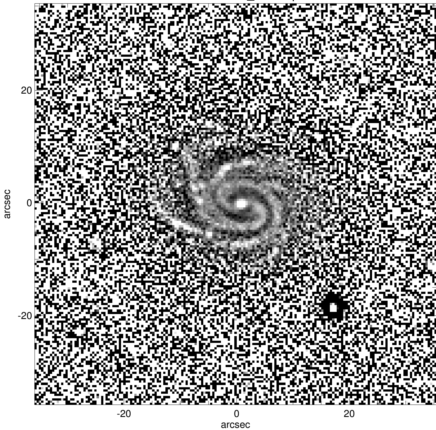
PGC0144600_unsharp
