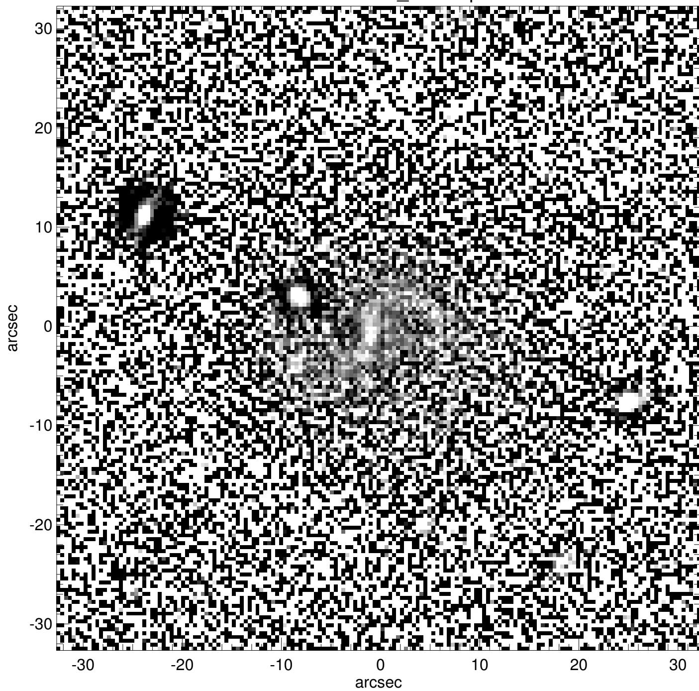
PGC0212869_unsharp
