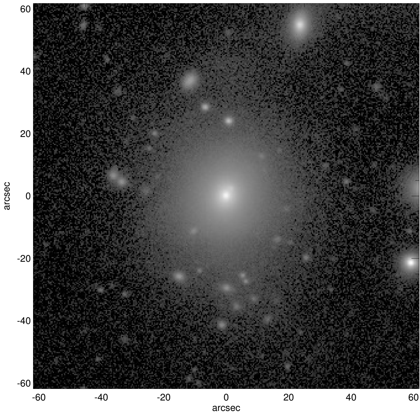
PGC1128372
