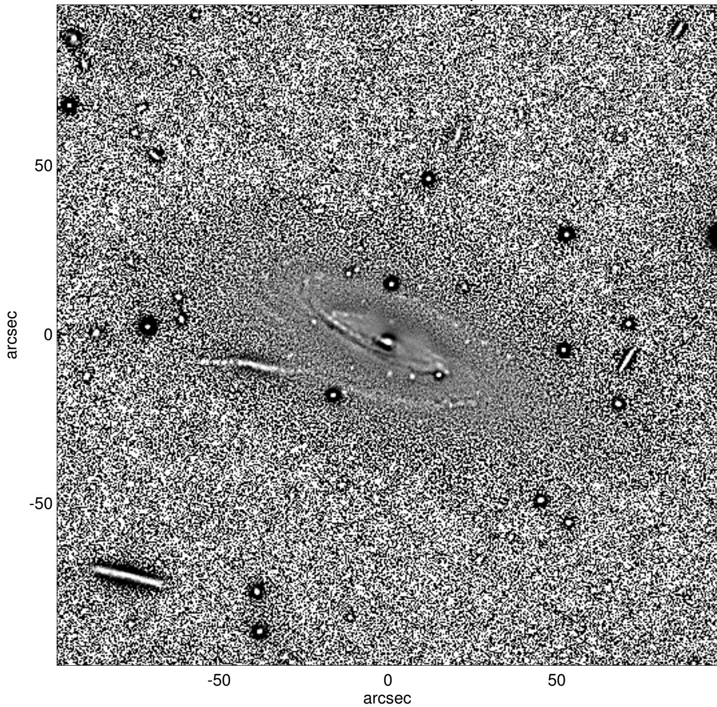
UGC02600_unsharp
