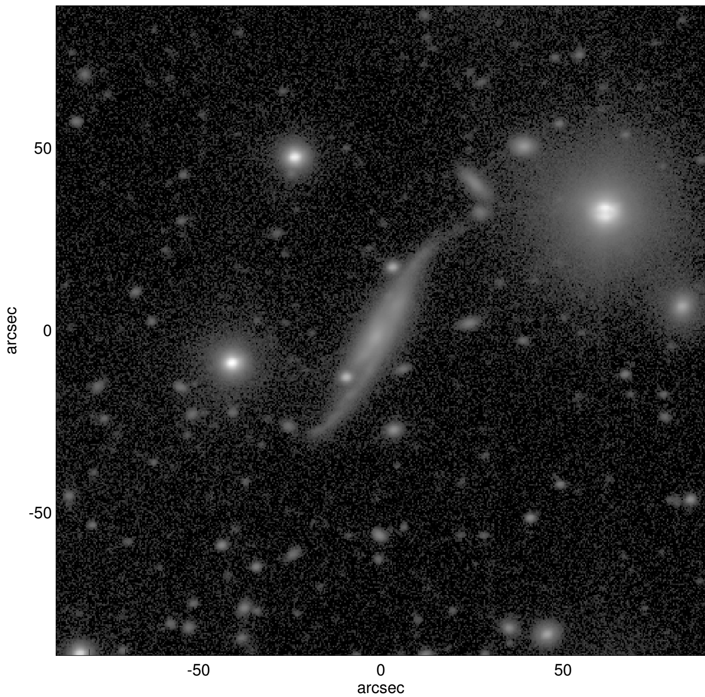
UGC12513
