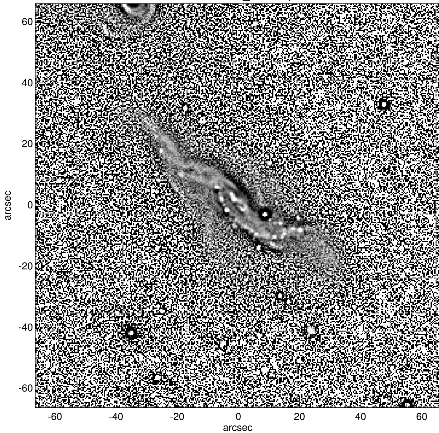
UGC12589_unsharp
