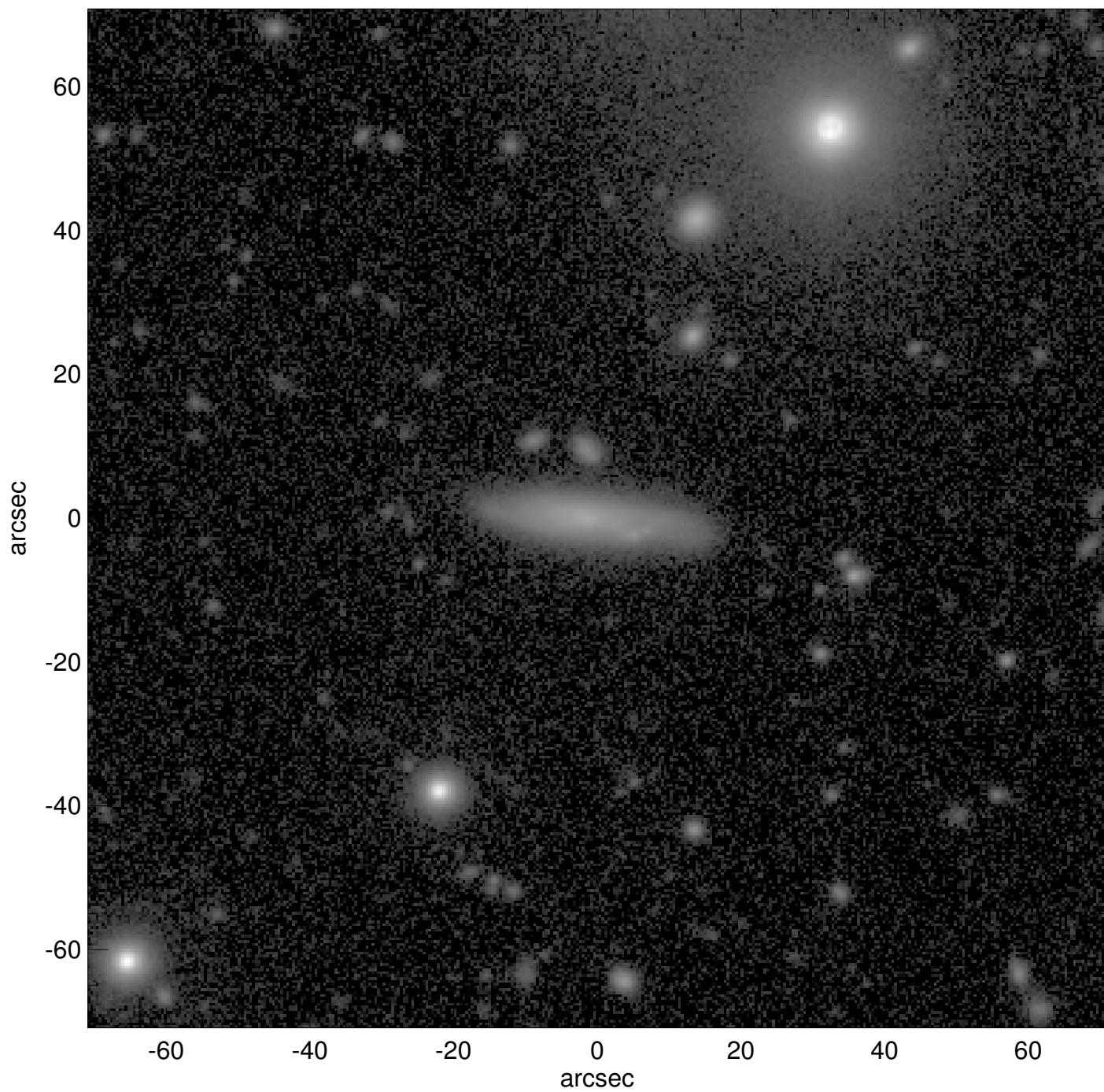
PGC1144533
