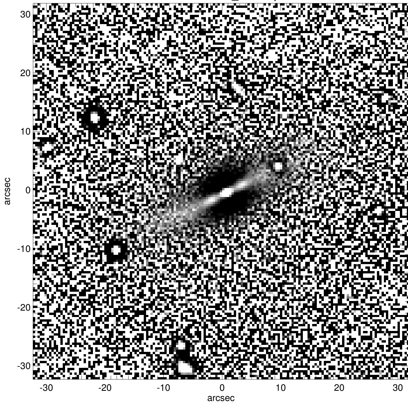
PGC3080526_unsharp
