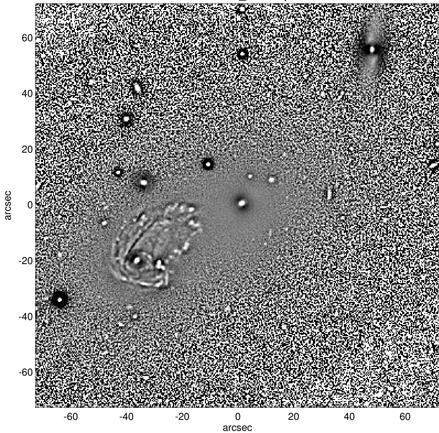
NGC1143_unsharp
