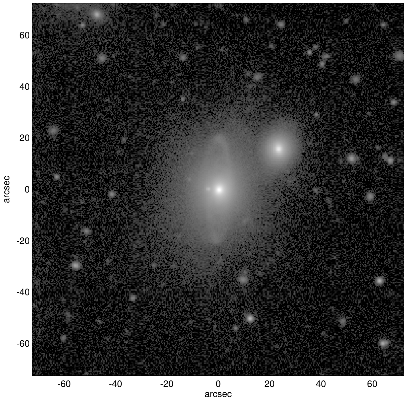
PGC1137934
