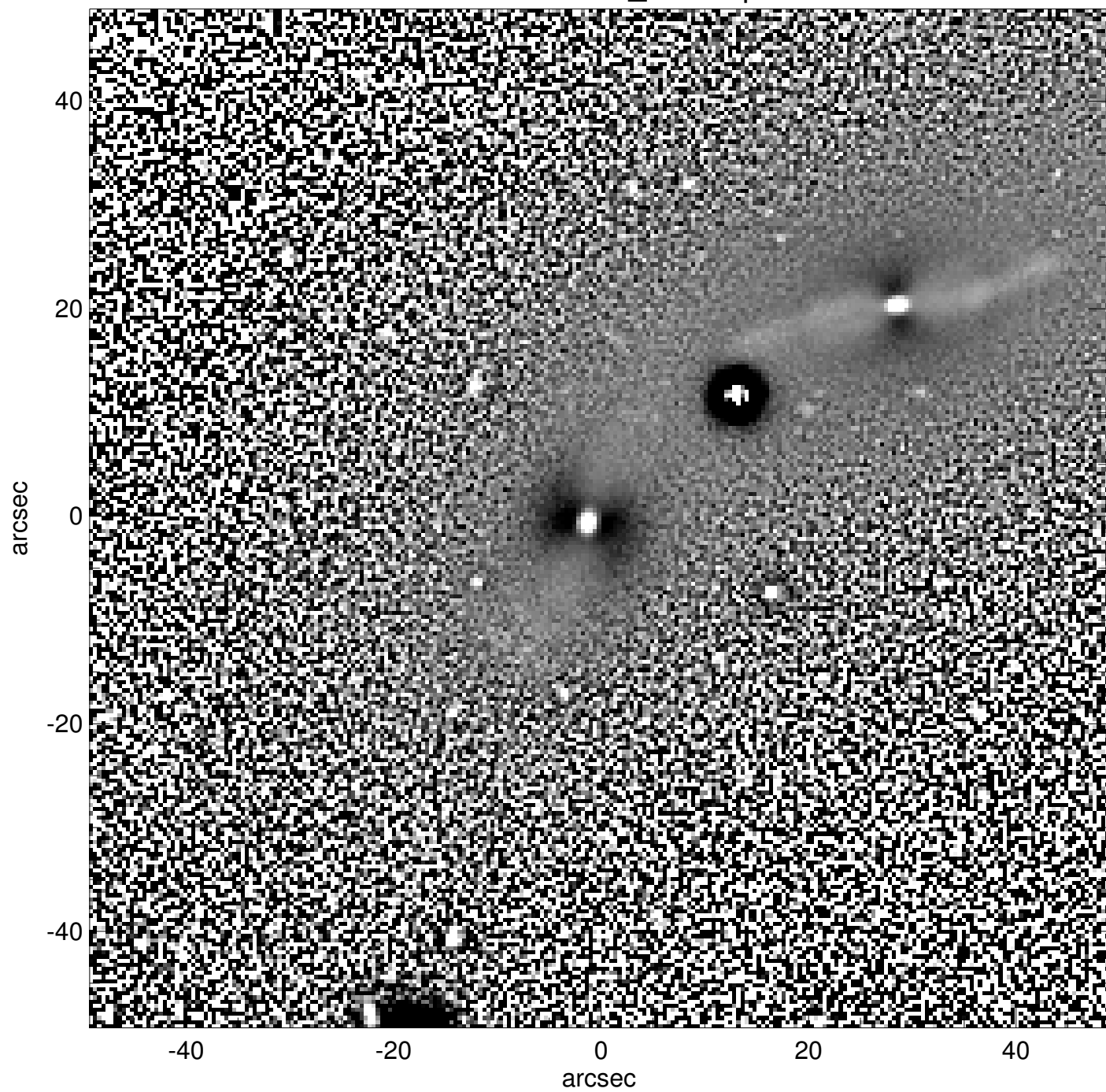
PGC0072808_unsharp
