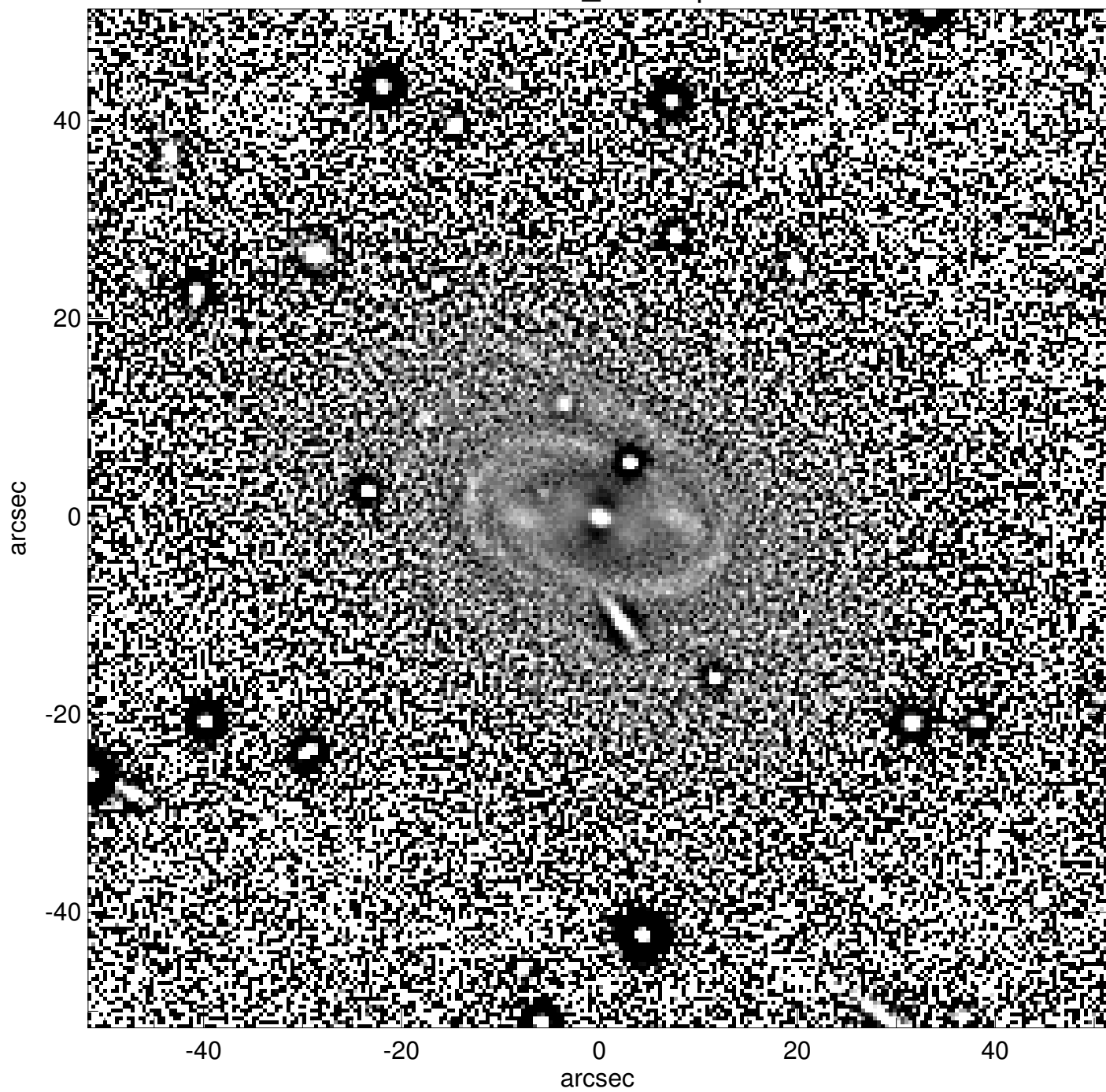
IC1381_unsharp
