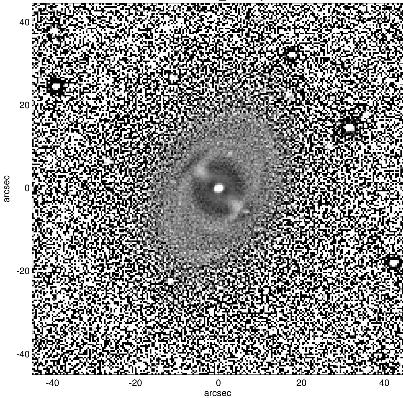
NGC7397_unsharp
