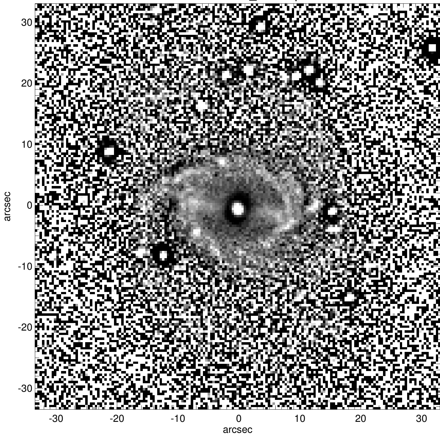
PGC1154257_unsharp
