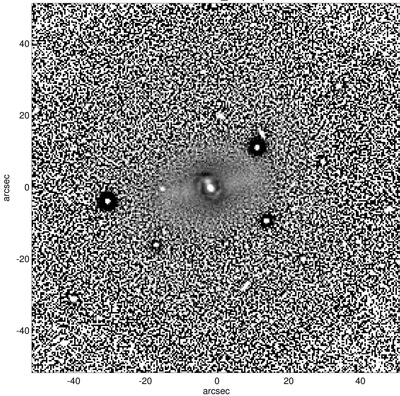
UGC00976_unsharp
