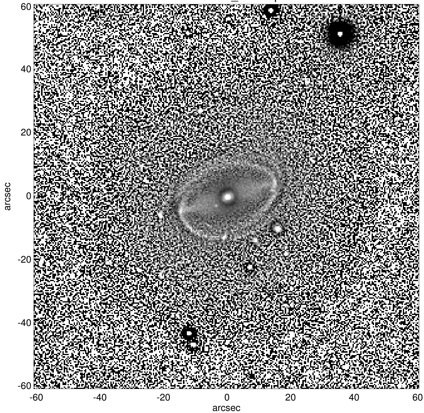
UGC01698_unsharp
