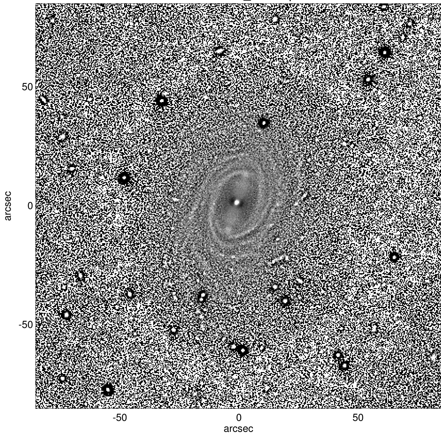
UGC02585_unsharp
