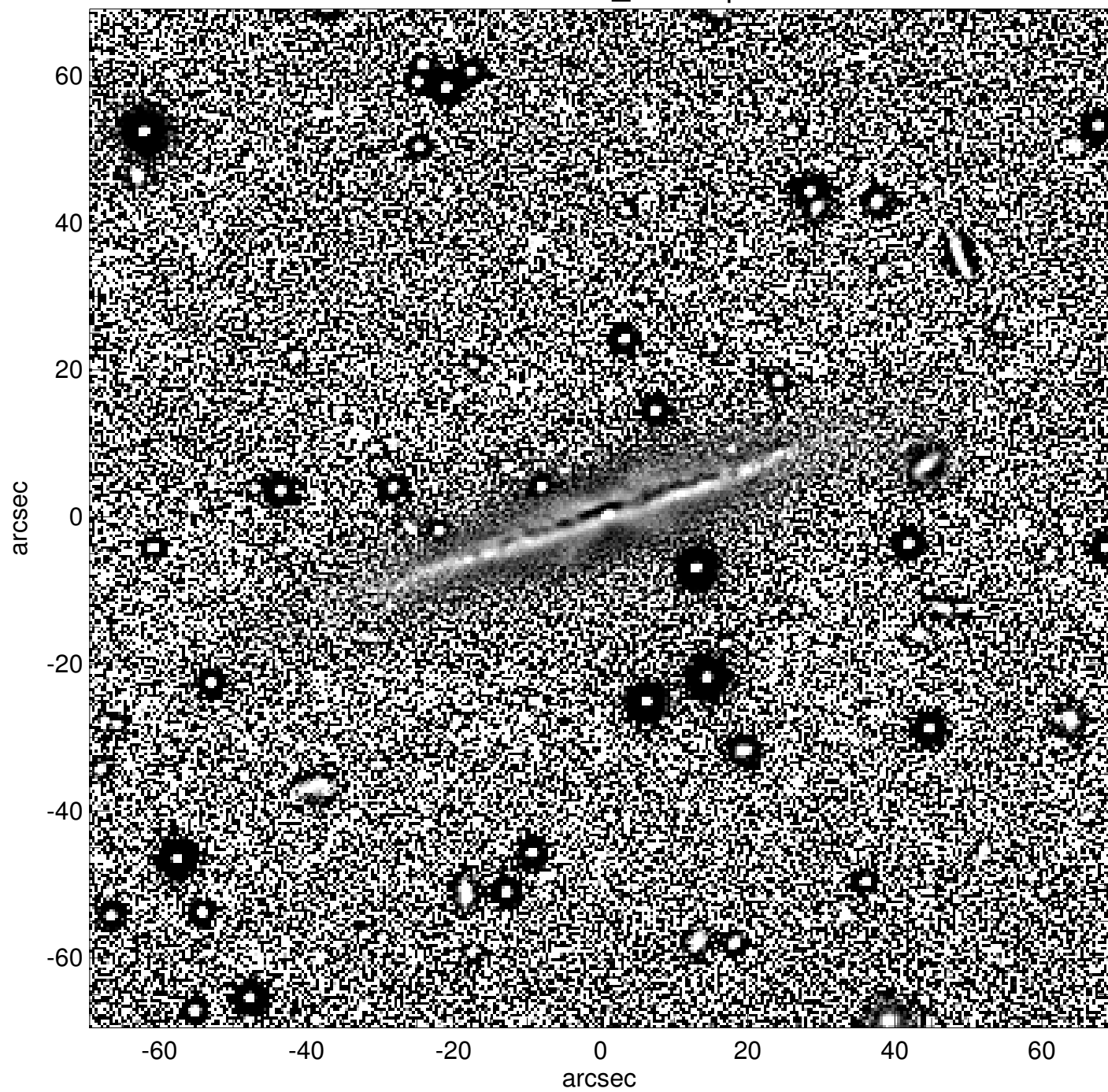
UGC11645_unsharp
