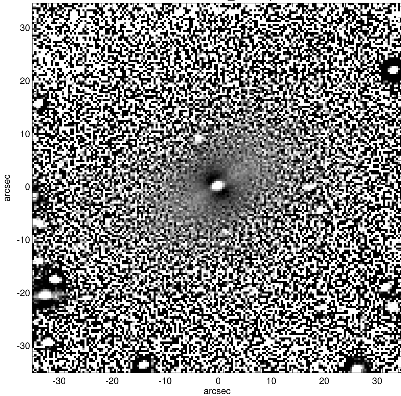
PGC1180786_unsharp
