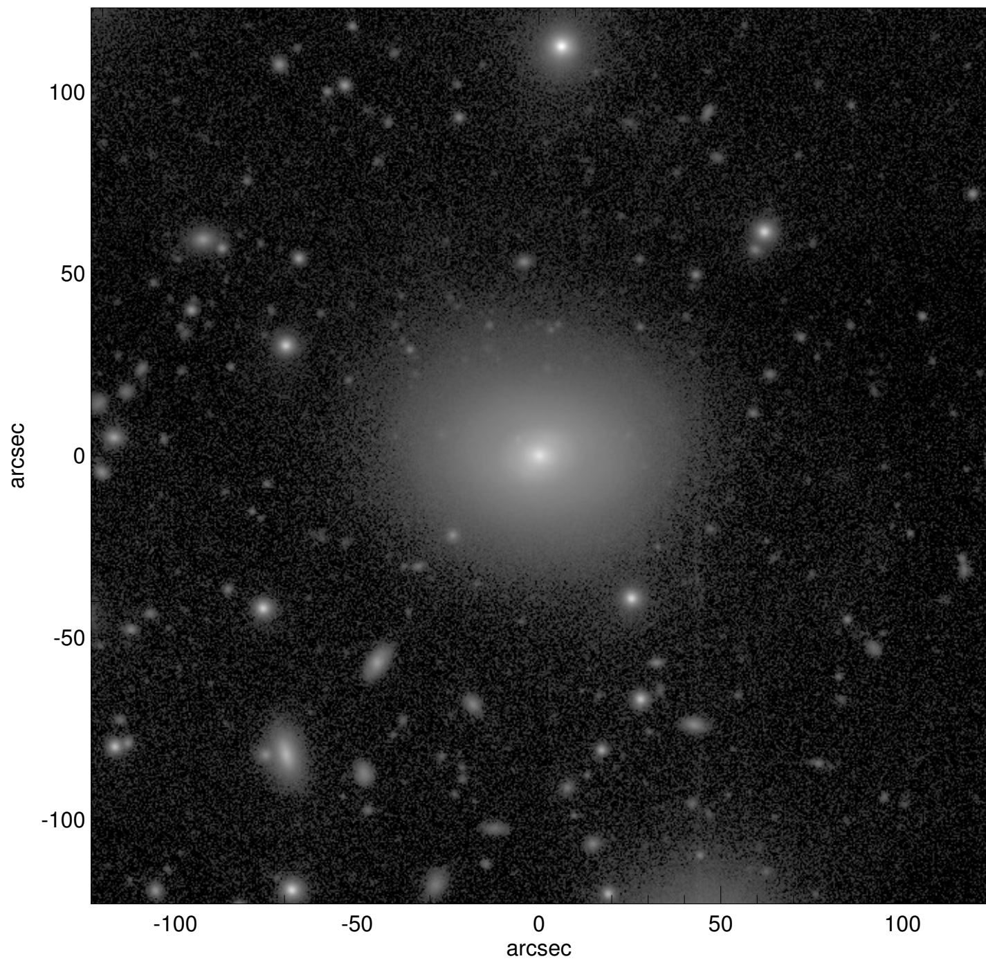
UGC12492
