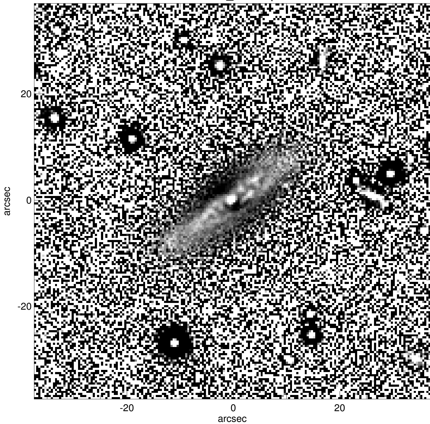
IC1383_unsharp
