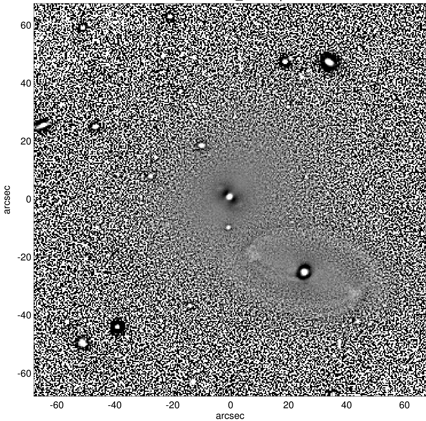
NGC0078B_unsharp
