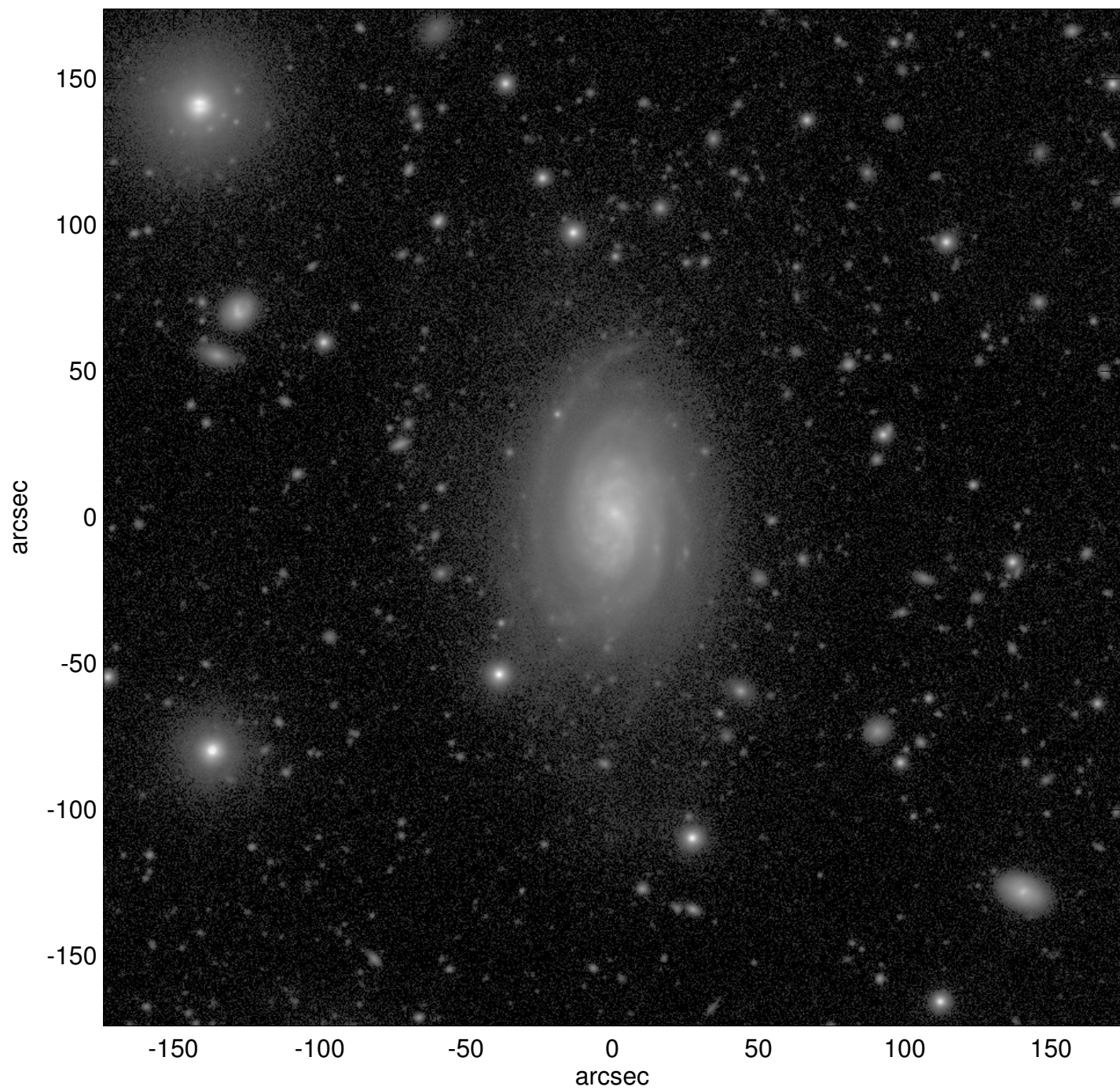
NGC0237
