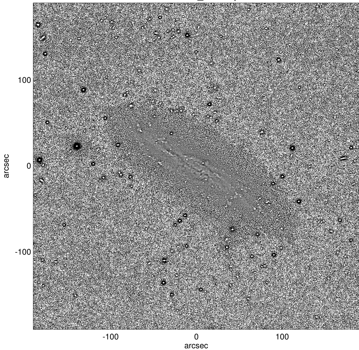
NGC0493_unsharp
