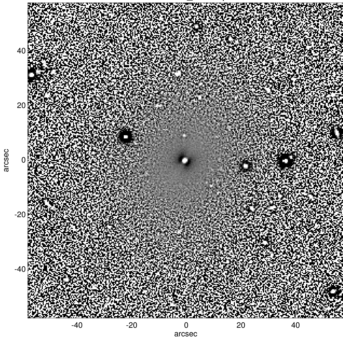
NGC0548_unsharp
