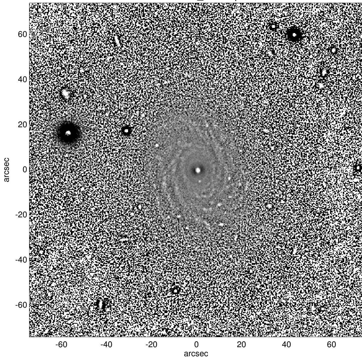
NGC0856_unsharp
