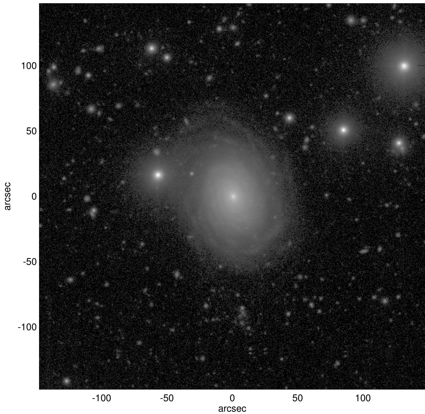
NGC0856
