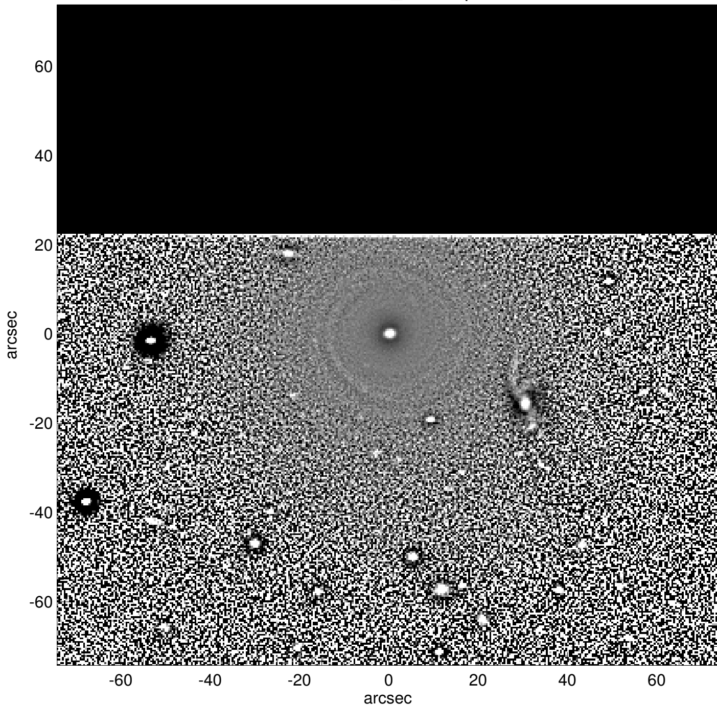
NGC0875_unsharp
