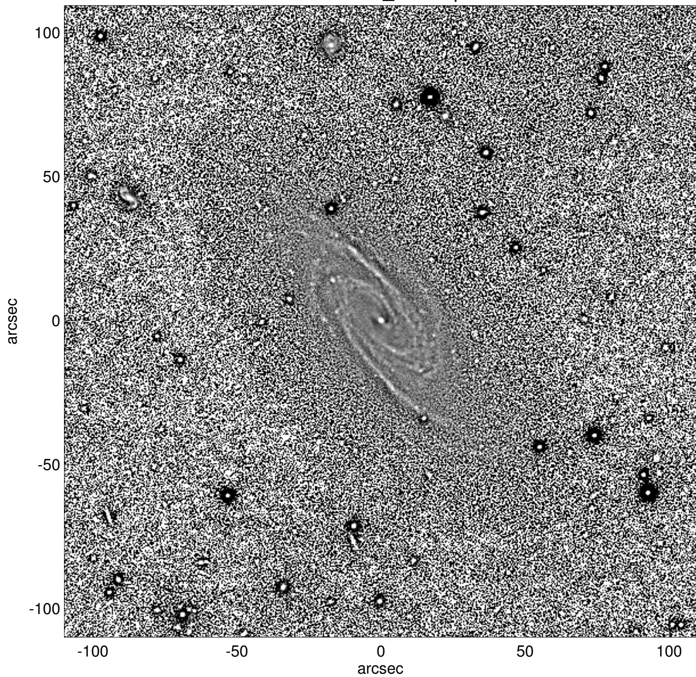
NGC0926_unsharp
