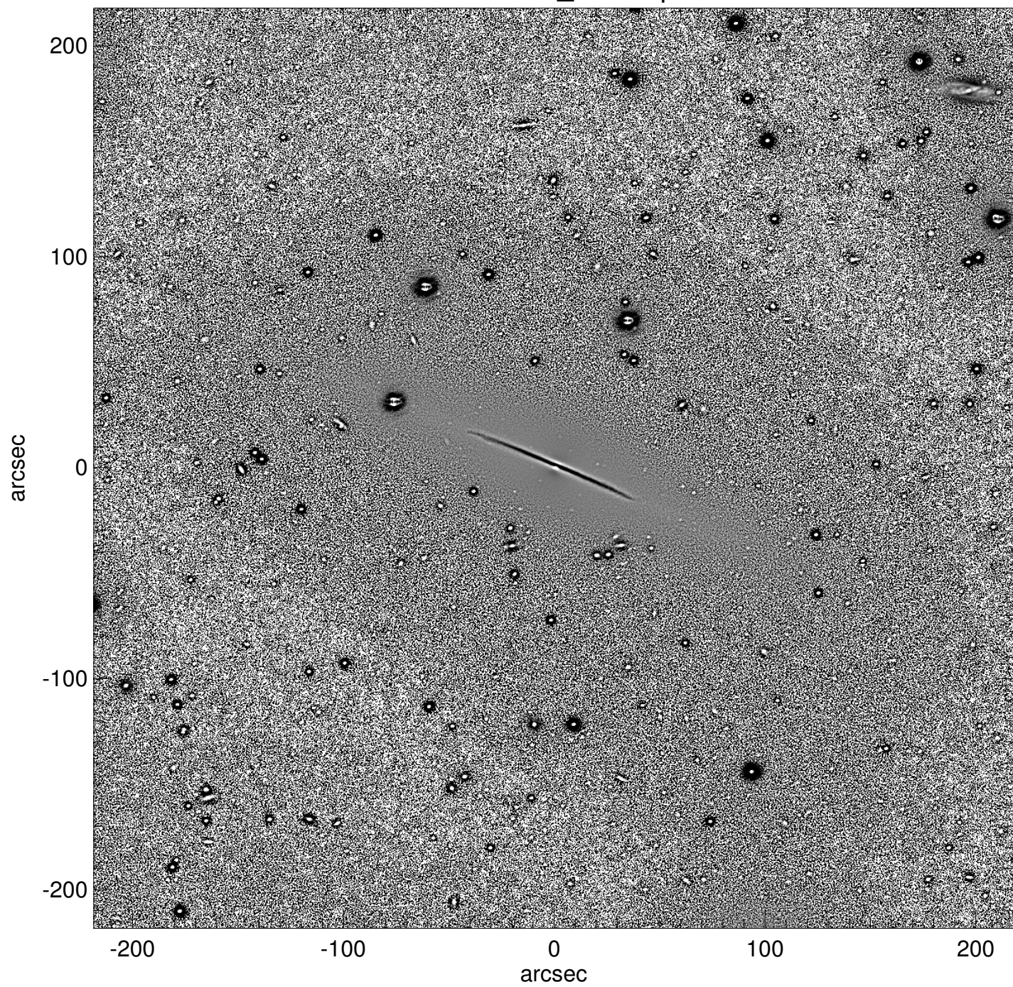
NGC1032_unsharp
