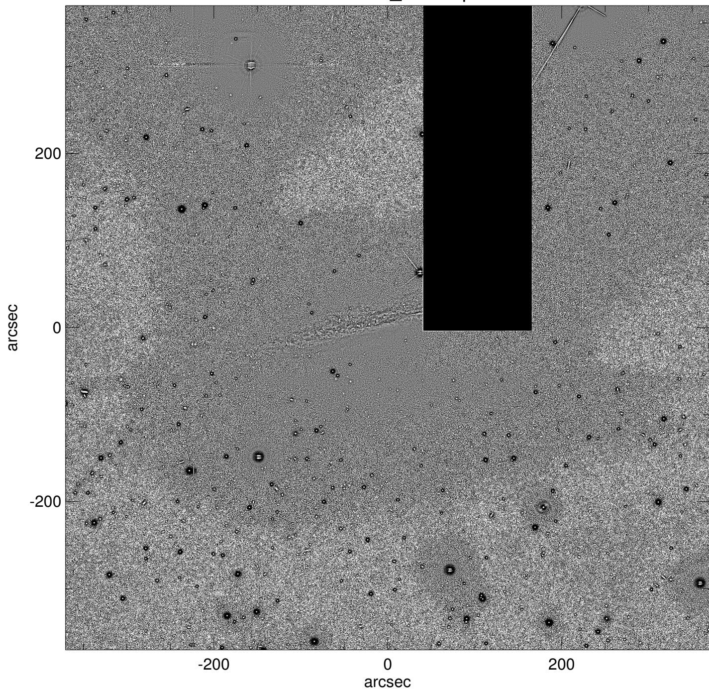
NGC1055_unsharp
