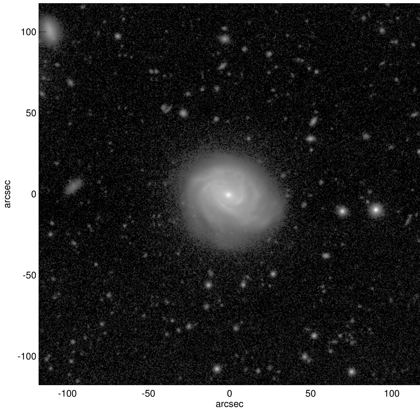
NGC1280
