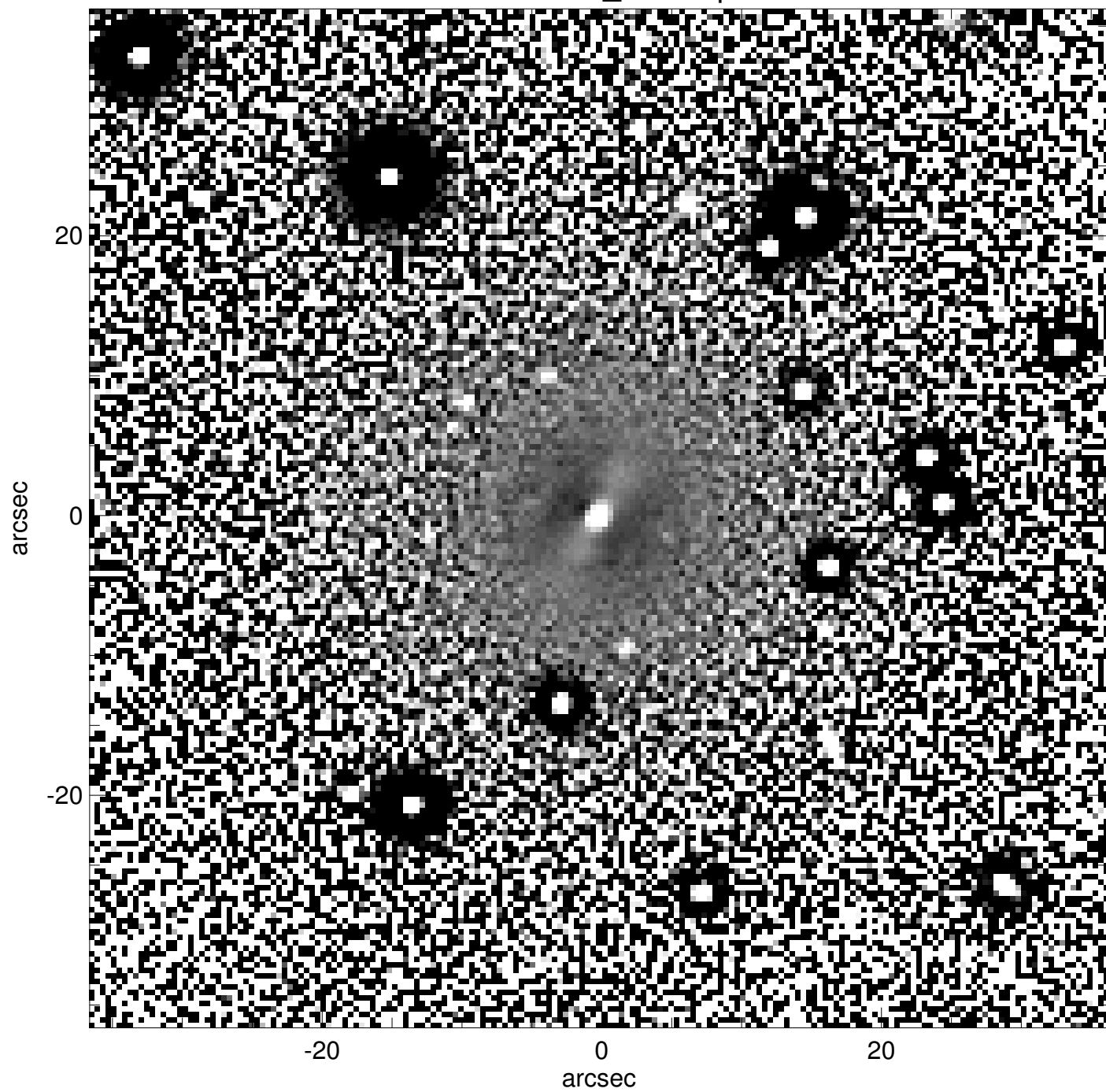
NGC6961_unsharp
