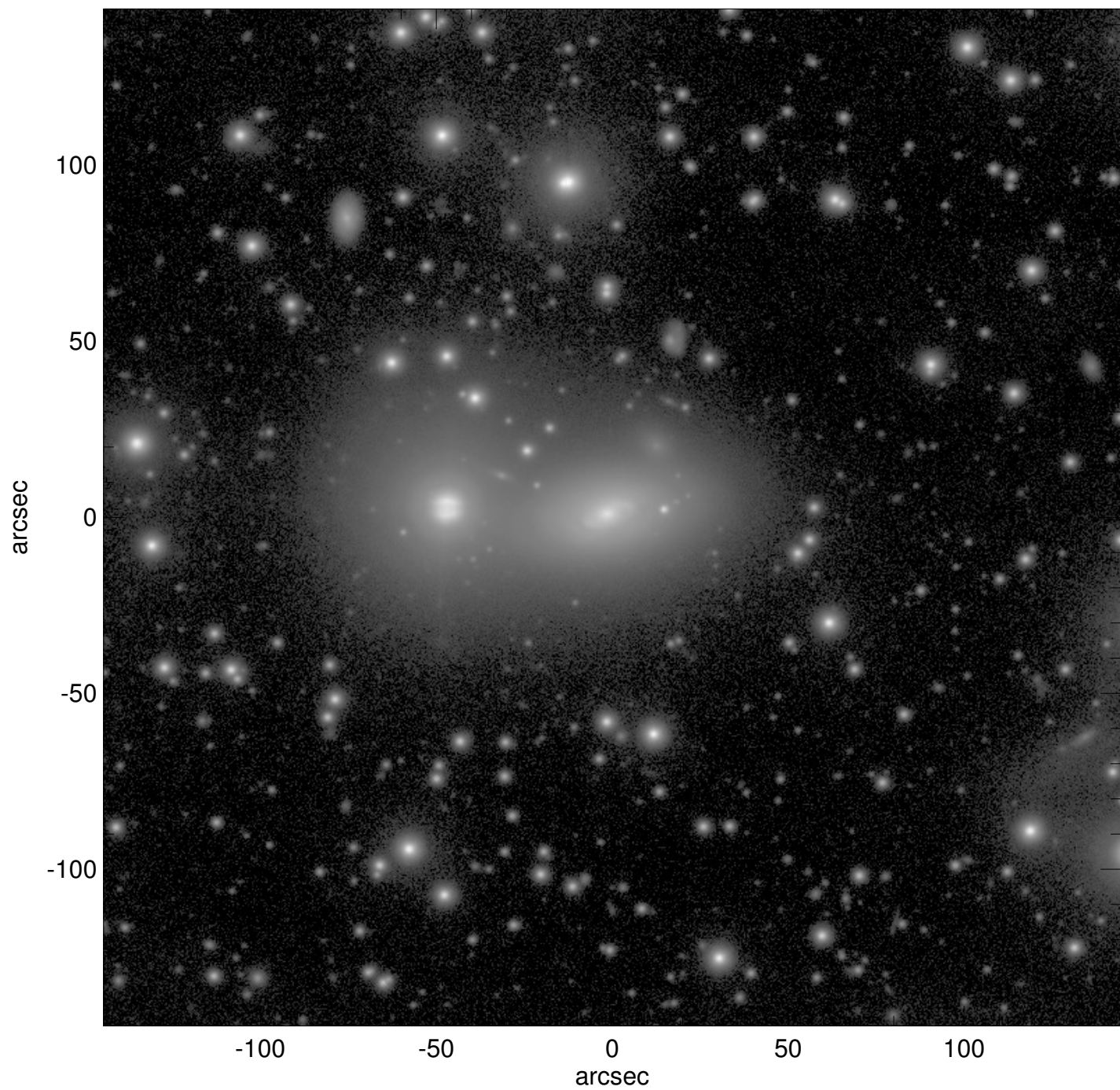
NGC6967
