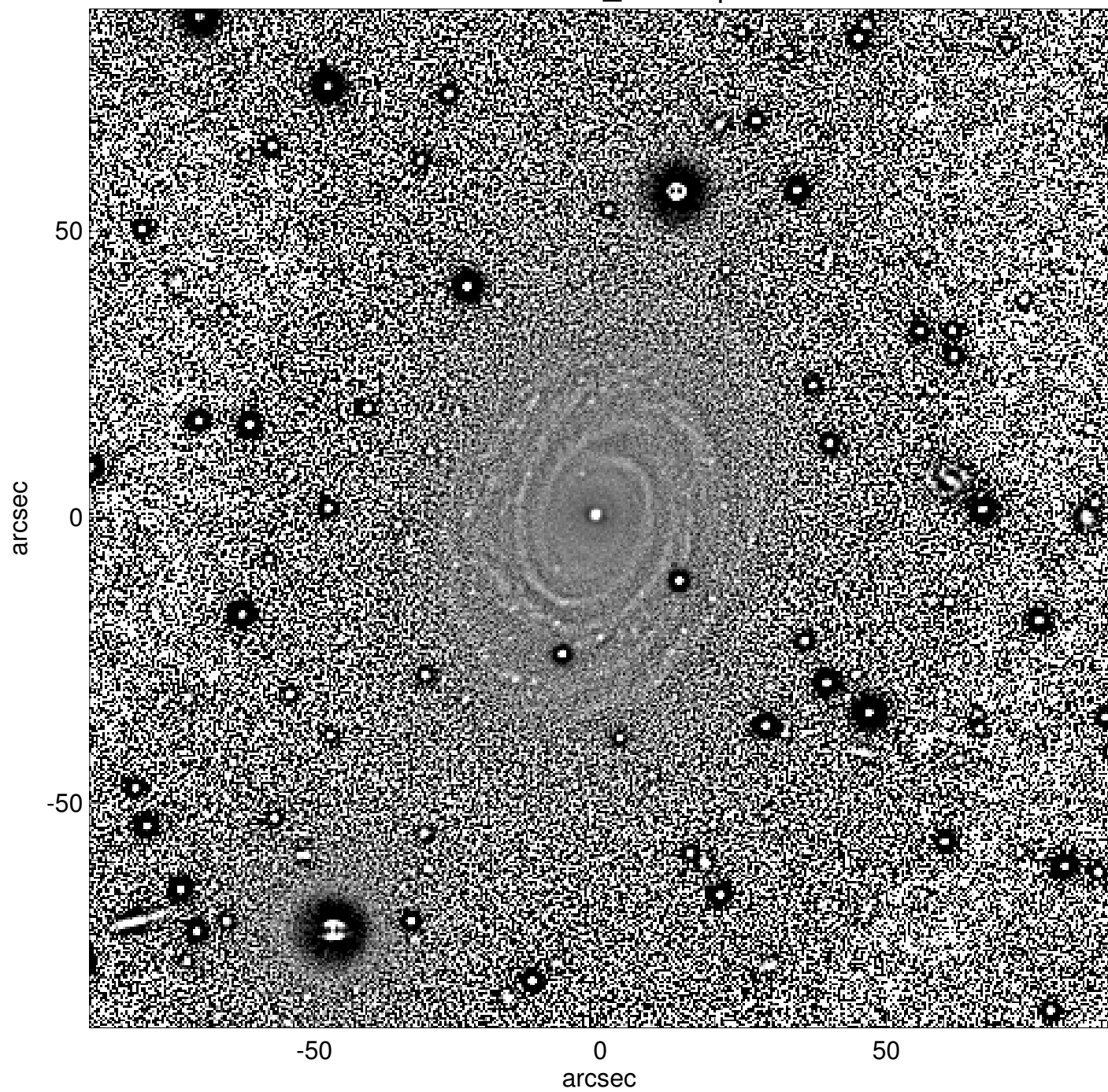
NGC7001_unsharp
