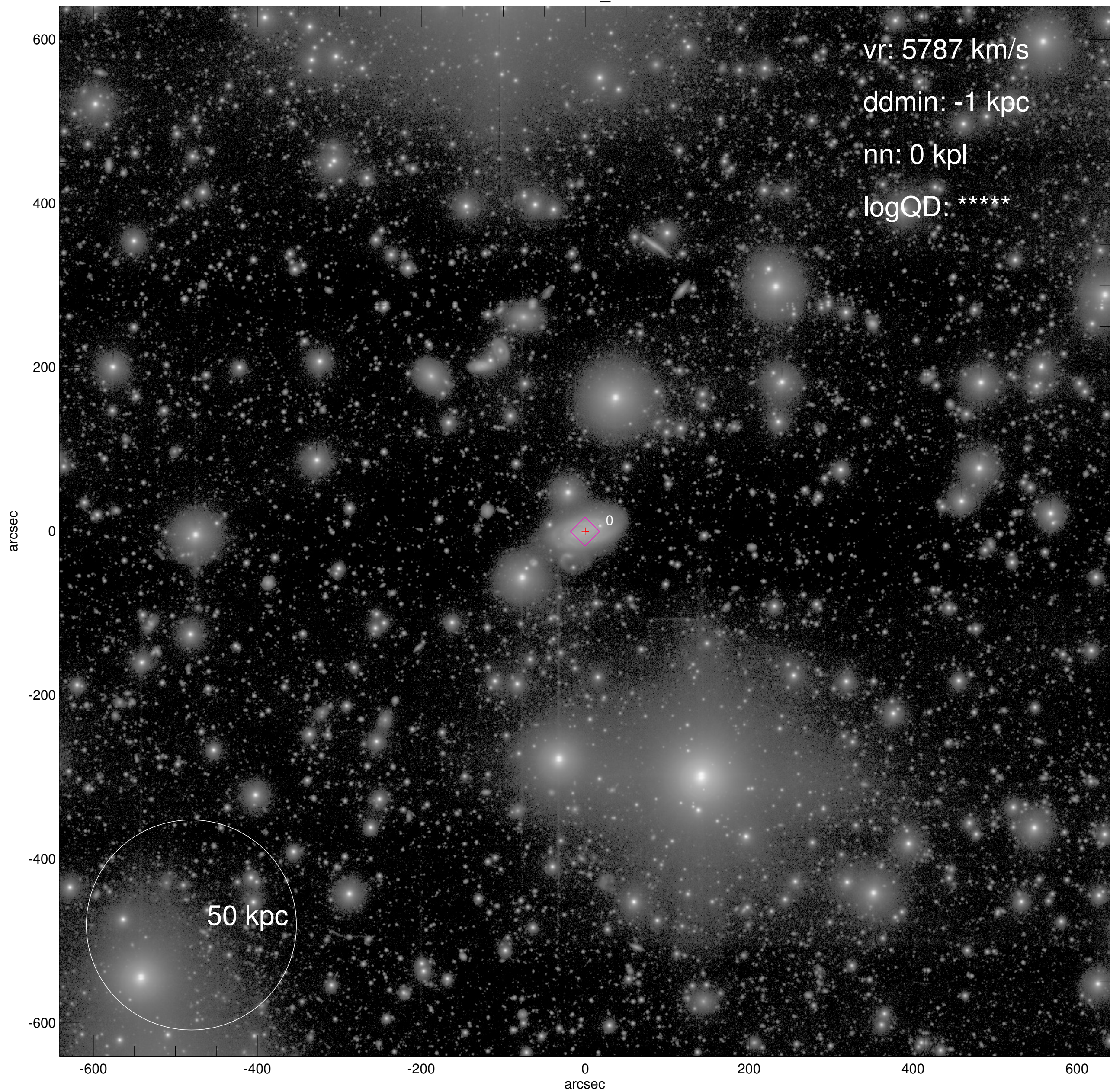
NGC7047_wide
